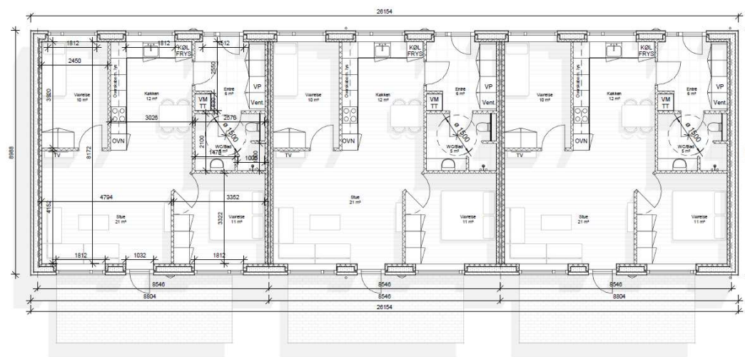
TYPE B (9m) 77m 2
