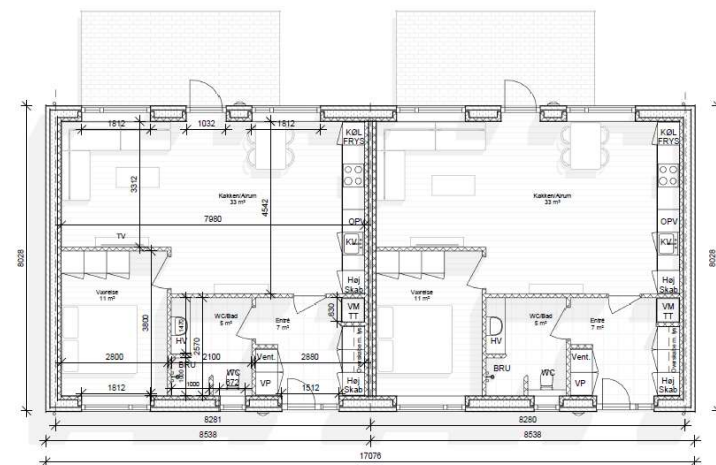
TYPE A (8m) 67m 2
